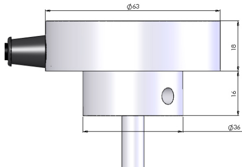
3271 SAE 5 BOLT Mount Unit Dimensions
