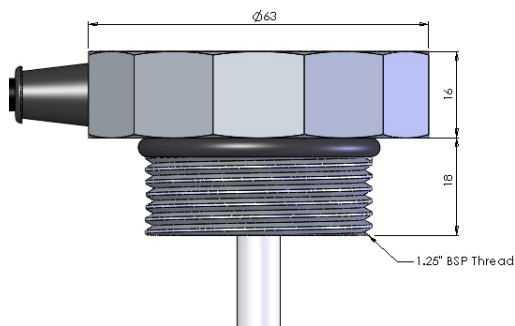
3271T 1 1/4" BSP Threaded Mount Unit Dimensions
